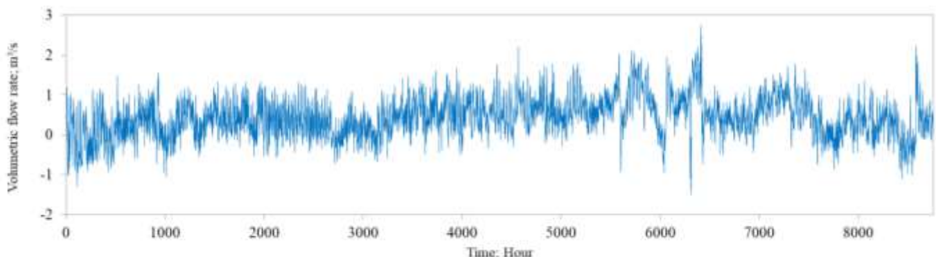
Fig.15: Instantaneous charge/discharge water volumetric flow to/from the upper reservoir in m³/s
